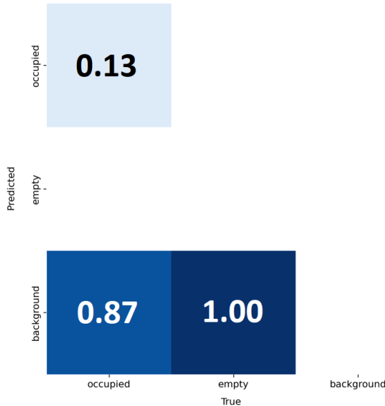
Figure 4. Confusion matrix of 50 epoch model
