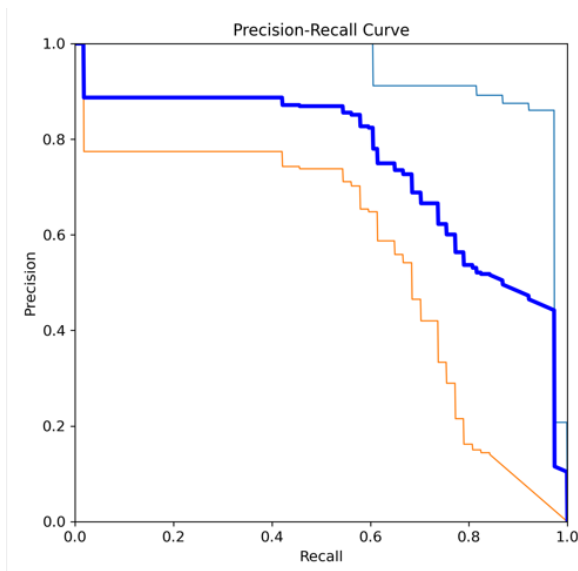
Figure 6. mAP graph of 50 epoch model
