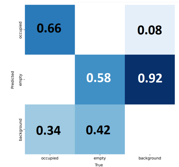
Figure 5. Confusion matrix of 300 epoch model
