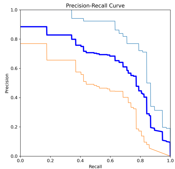
Figure 7. mAP graph of 300 epoch model
