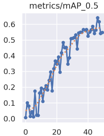
Figure 6. mAP graph of 50 epoch model
