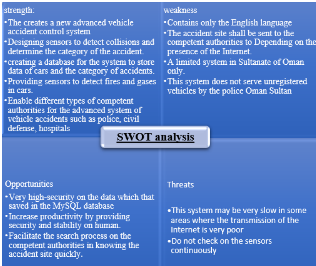
Figure 1. SWOT analysis
